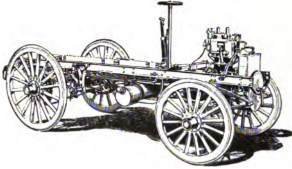
FIG. 376.—Running Gear of the Heavy Delivery Wagons manufactured by the American Daimler Co., showing the motor and machinery in position.
